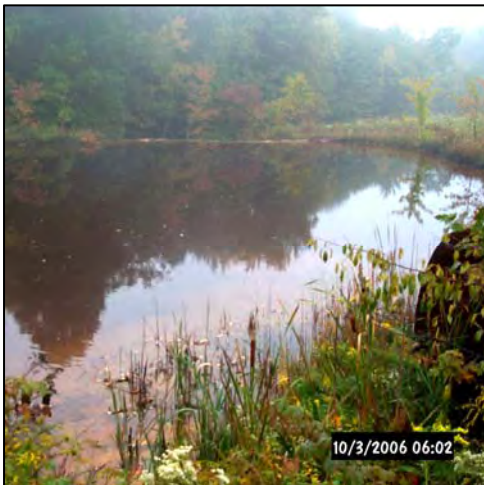
Existing treatment pond TB1 (Left) receives mine discharges MC1, MC2, and MC3 which emanate from the "McIntire" site. The effluent of TB1 (Right) used to be the headwaters of tributary #15. The natural formation of iron minerals at low pH, plugging old piping (Center), has been incorporated into the passive system design.
