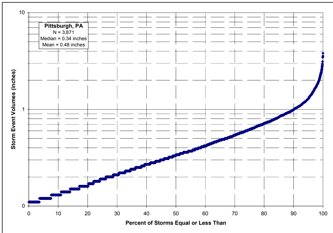
Figure 3-4: Probability Distribution of Storm Event Volumes (PIA Historic Record)
