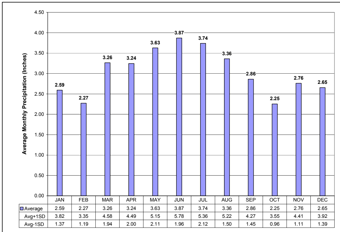
Figure 3-2: Average Monthly Precipitation Volumes (PIA Historical Record)
