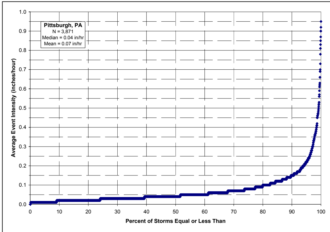
Figure 3-6: Probability Distribution of Average Event Intensity (PIA Historic Record)
