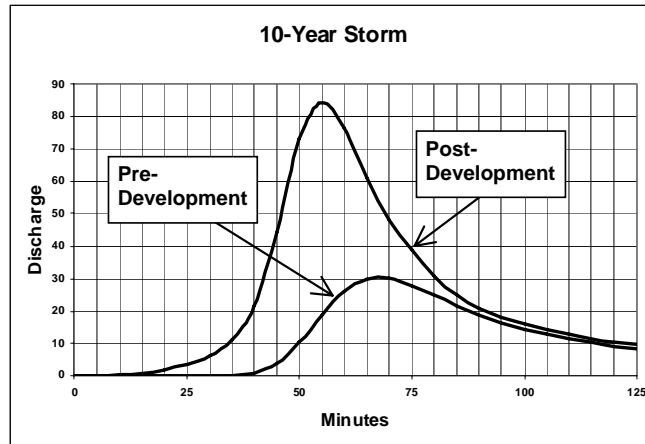
Figure 4.3 - Hydrograph under Pre- and Post Development Conditions
