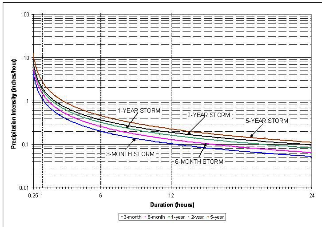
Figure 3-9: Intensity-Duration-Frequency Curve (PIA Historic Record)
