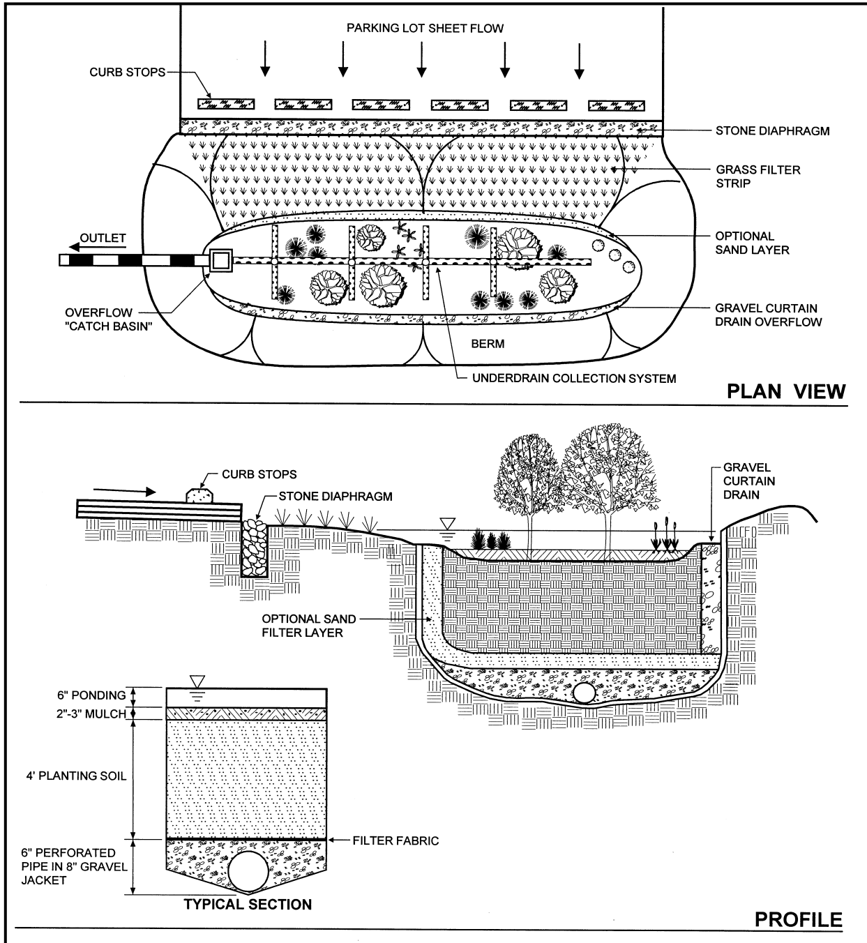
Schematic of a Typical On-line Bioretention Area
