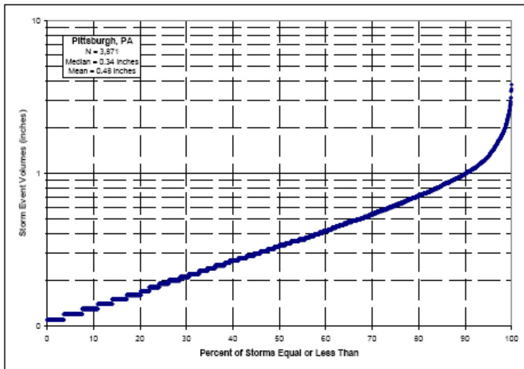
Figure 5.3 Synoptic Precipitation Analysis for the ALCOSAN Service Area
