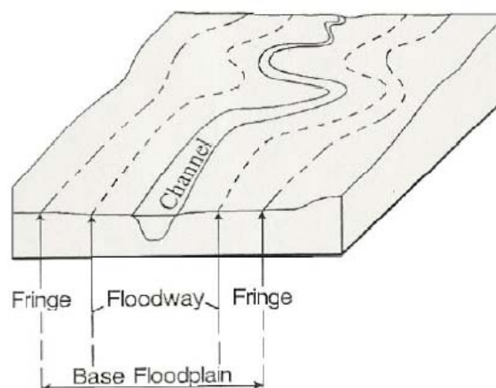
Figure 6.3 Floodway Section
