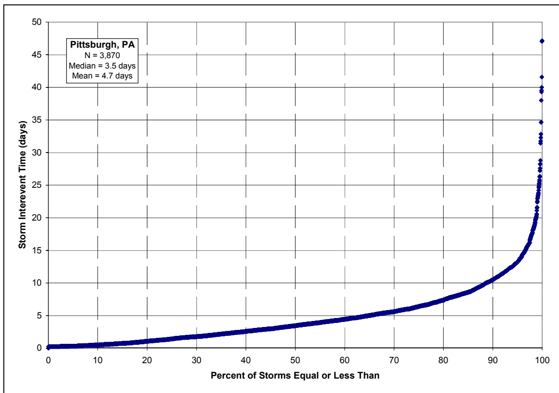
Figure 3-8: Probability Distribution of Storm Interevent Time (PIA Historic Record)
