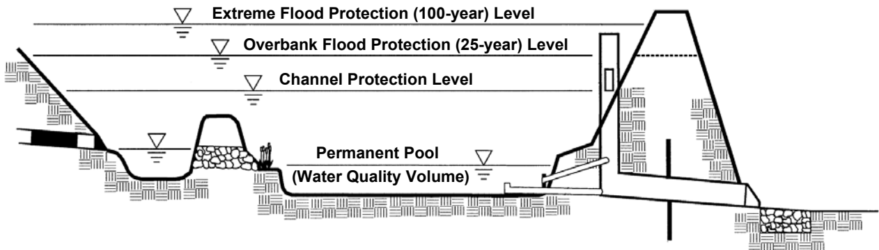
Figure 5.2 - Unified Sizing Criteria Water Surface Elevations in a Stormwater (Wet) Pond From the Georgia Stormwater Management Manual
