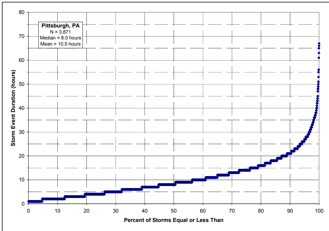
Figure 3-5: Probability Distribution of Storm Event Durations (PIA Historic Record)
