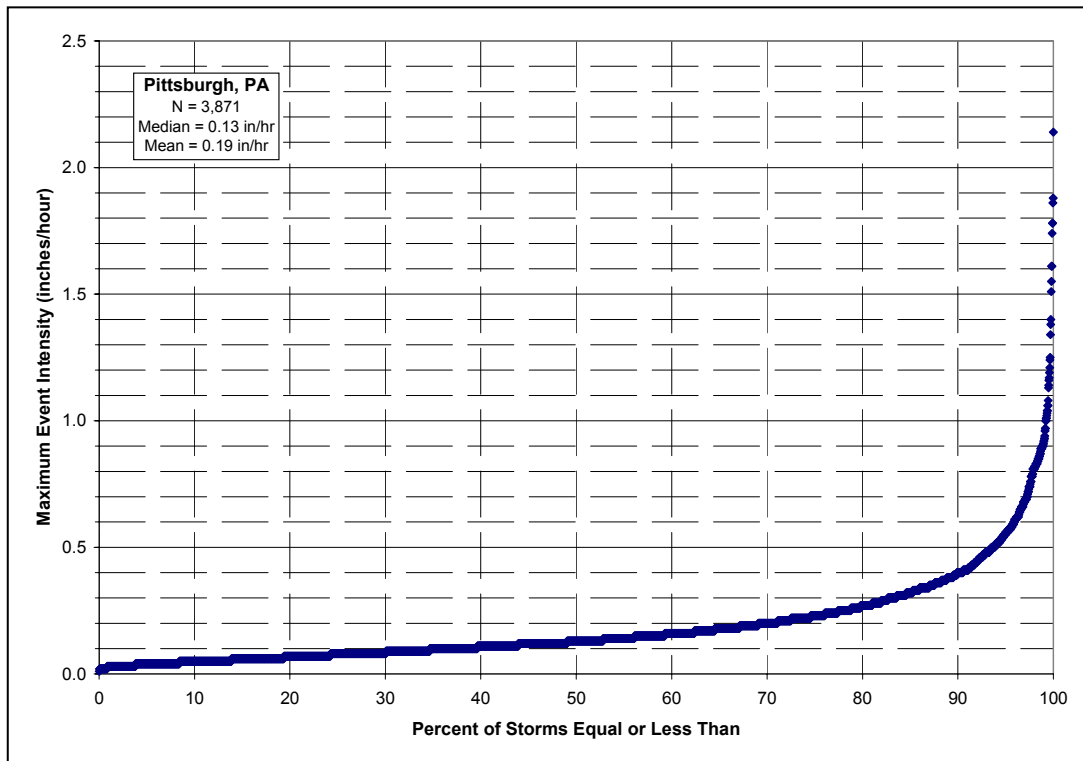
Figure 3-7: Probability Distribution of Maximum Event Intensity (PIA Historic Rec.)
