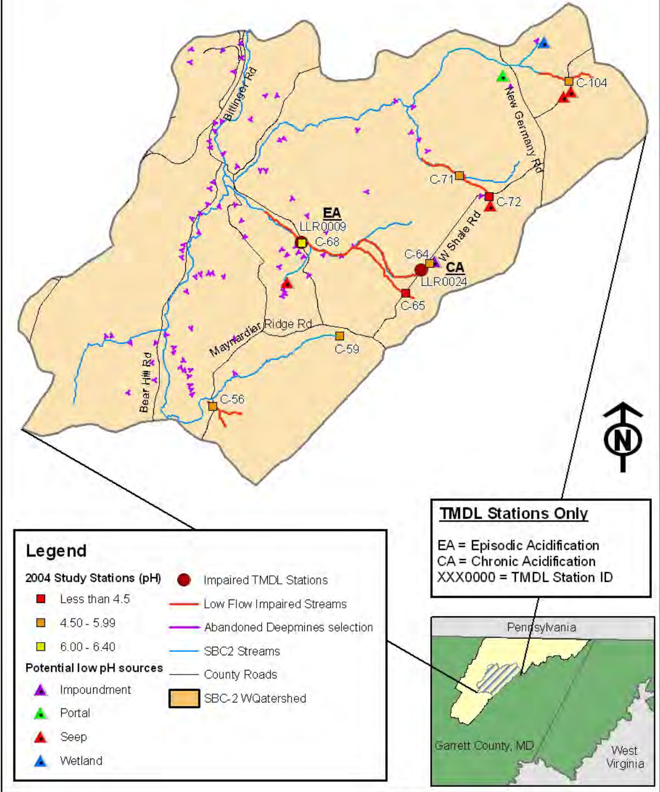
Figure 14. SBC-2 Watershed Low Flow Impairment Sources
